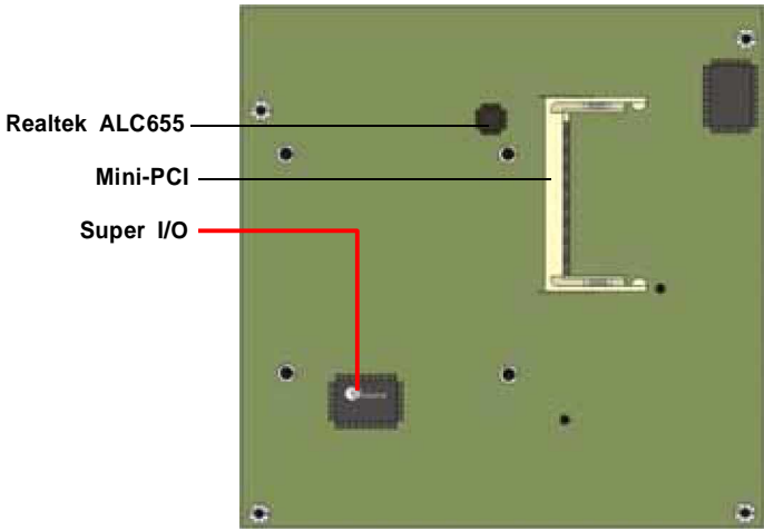
(Solder Side)
