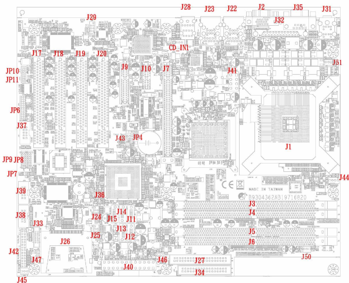
Figure 2-1 2801290 Jumper & Connector Location
