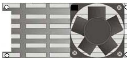
LP-172D5 Heatsink with Fan x 1 (OHS-172F)/ (2181010013)
