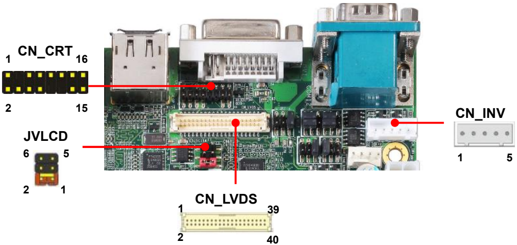
CN_CRT: CRT 16-pin connector (Pitch 2.00 mm)
