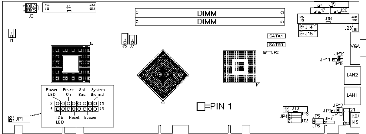
Figure 2-1: Jumper Location
