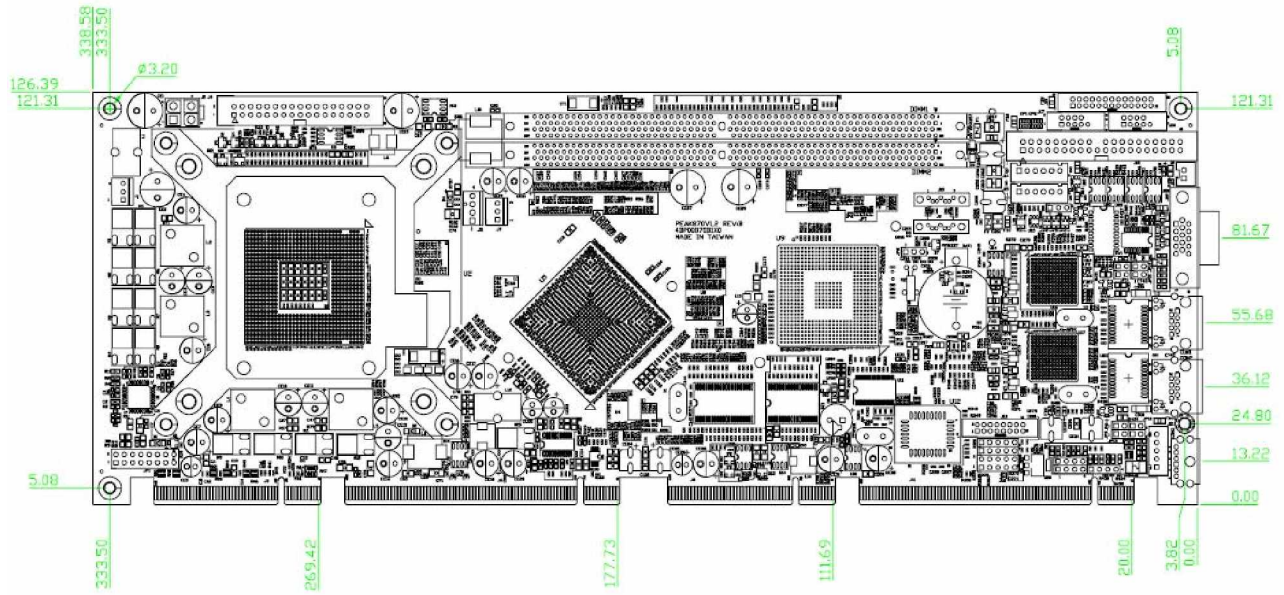
Figure 1.3: Mechanical Drawing of the 3301520
