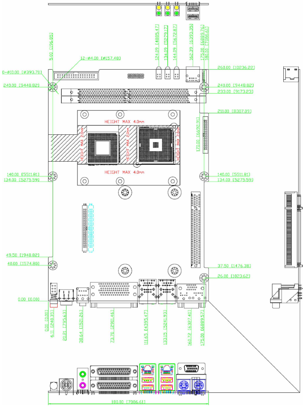
Figure 1.2: Mechanical Drawing of the 3302000
