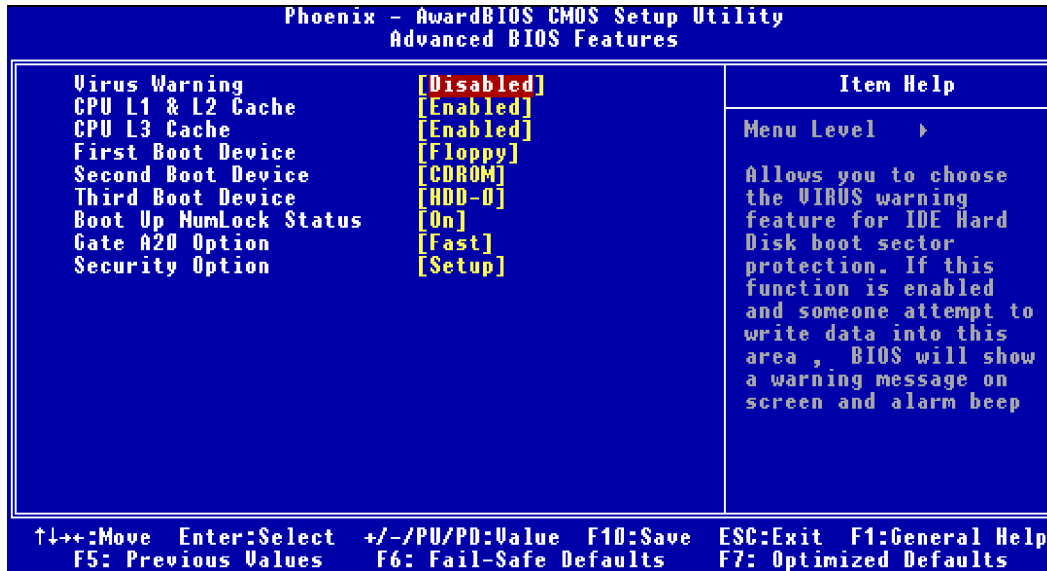
Figure 4-3: BIOS – Advanced BIOS Features
