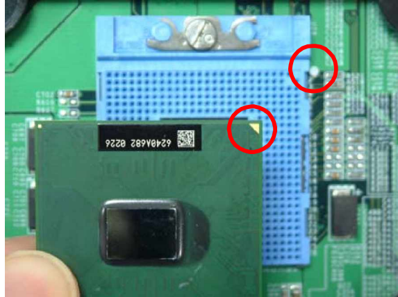
Figure 3-7: How to Install CPU (1)
