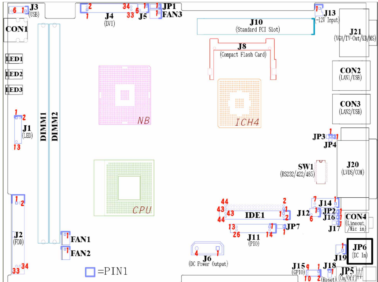
Figure 2-1: Jumper Location
