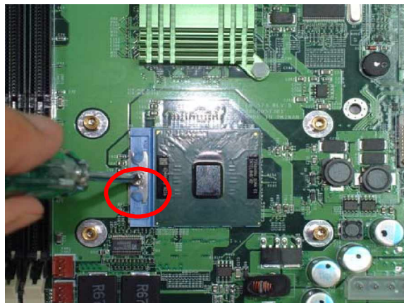
Figure 3-8: How to Install CPU (2)
