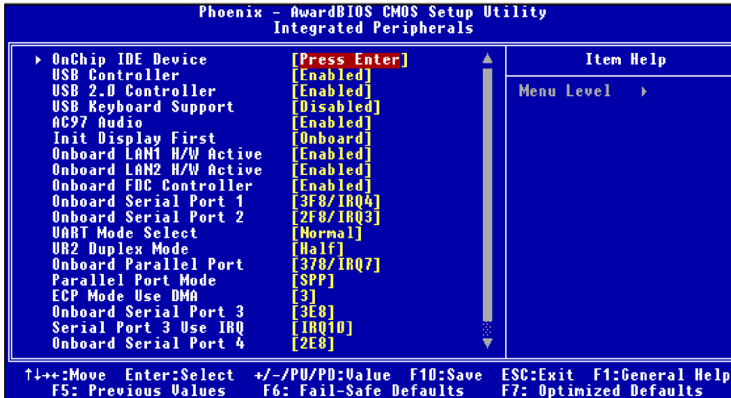
Figure 4-5: BIOS – Integrated Peripherals
