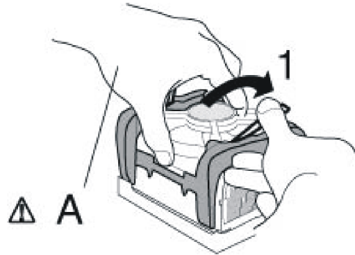
Figure 3-12b: Installing the Fan Heatsink (5) Close Clip Lever (1). While Holding the Topside of Fan Heatsink (A)
