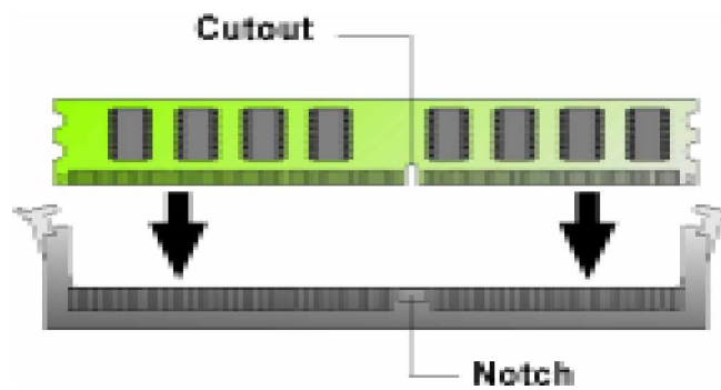
Figure 3-2: How to Install DIMM (2)
