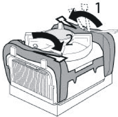
Figure 3-12a: Installing the Fan Heatsink (4) Close Clip Levers. One at a Time
