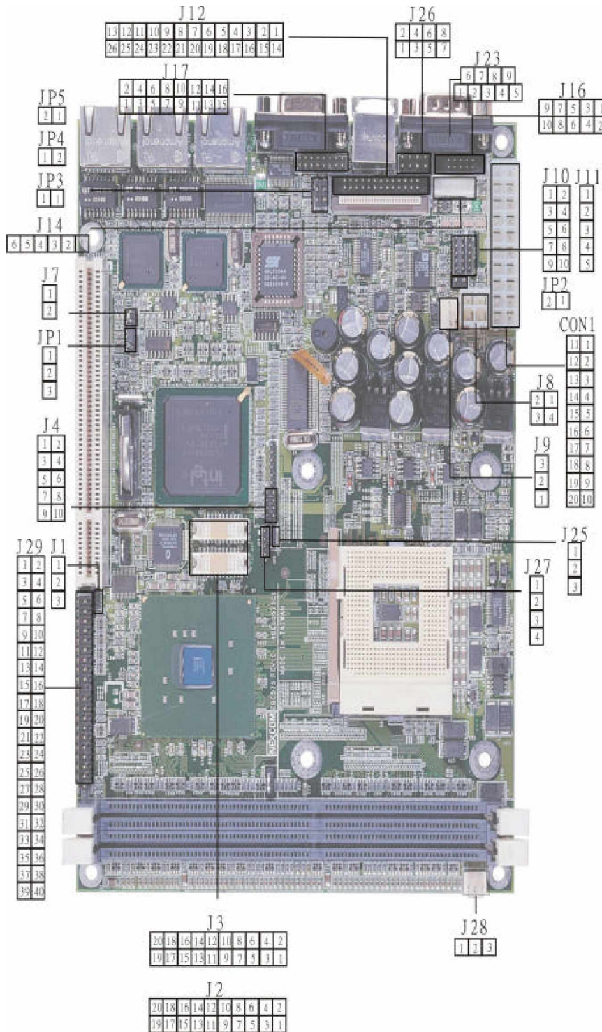
Figure 2-1: 3302010 Board Main Jumpers and Switches
