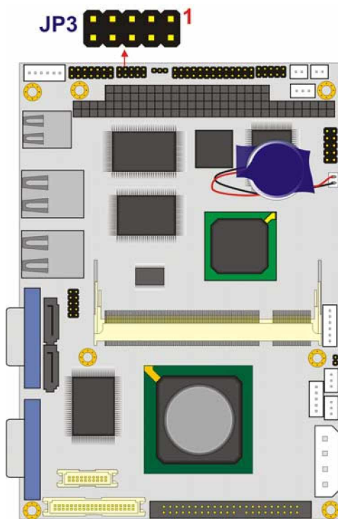
Figure 4-5: COM 1/2 Port RI and Voltage Select Jumper Pinout Locations
