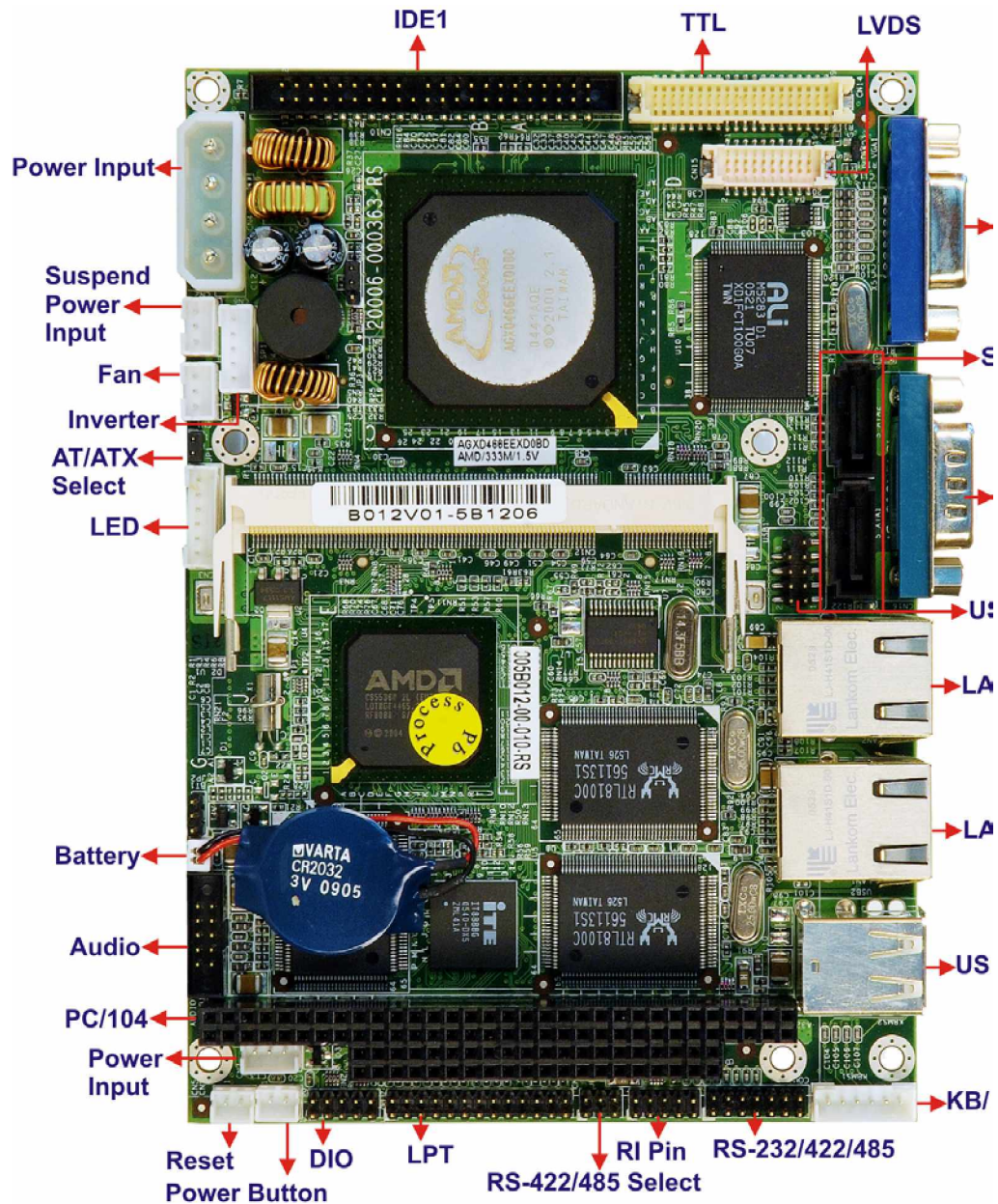
Figure 1-1: 3302040 Overview
