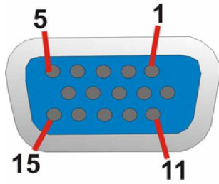
Figure 3-26: VGA1 Connector
