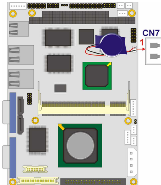
Figure 4-2: Clear CMOS Connector
