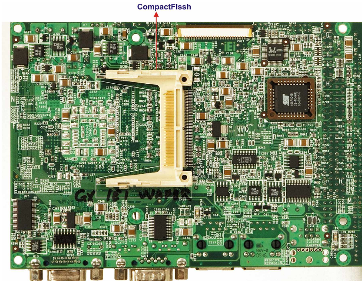
Figure 1-2: 3302040 Solder Side Overview
