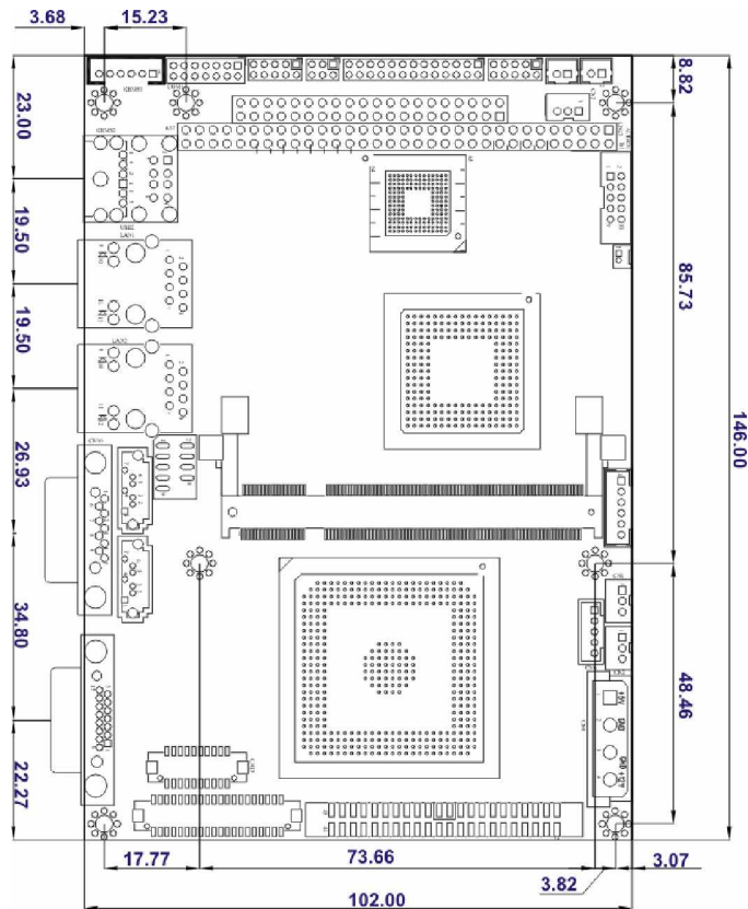
Figure 2-1: 3302040 Dimensions (mm)
