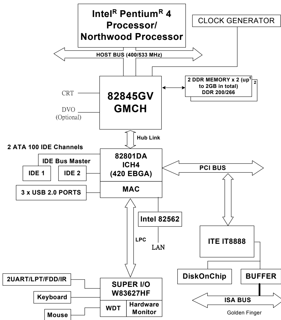
3307421 System Block Diagram
