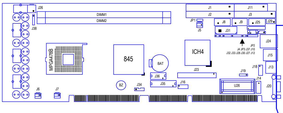
Figure 2-1 3307421 Jumper/Connector Location
