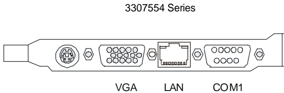
Figure 1: I/O bracket layout
