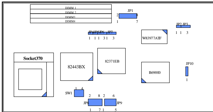
Figure 2-1 3307555 Jumper Locations
