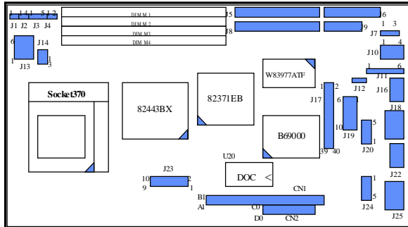
Figure 2-2 3307555 Connector Locations
