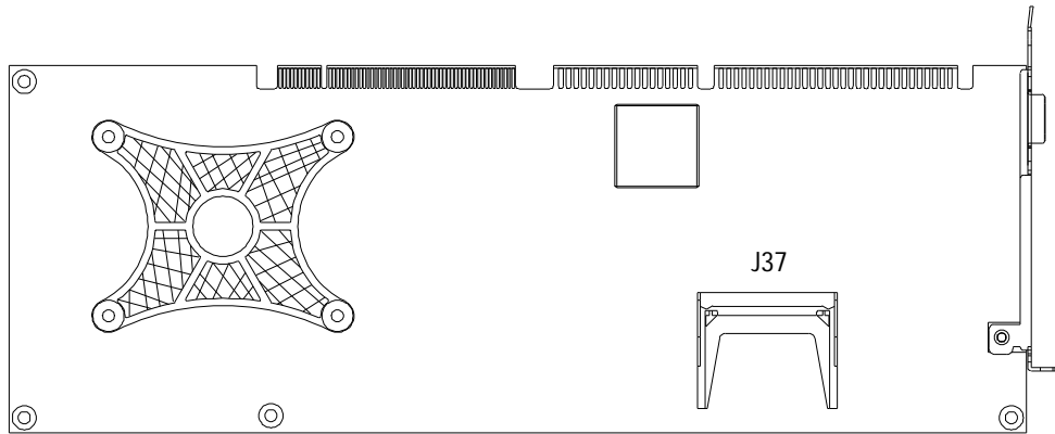
Figure 2-1 3307559 Jumper Location
